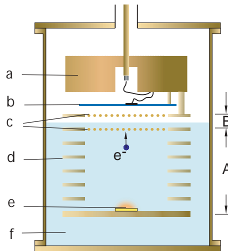
Figure 1. Experimental setup. a, helium free stage. b, calorimeter. c, grid electrodes. d, drifting field electrode rings. e, electron source. f, superfluid helium.
