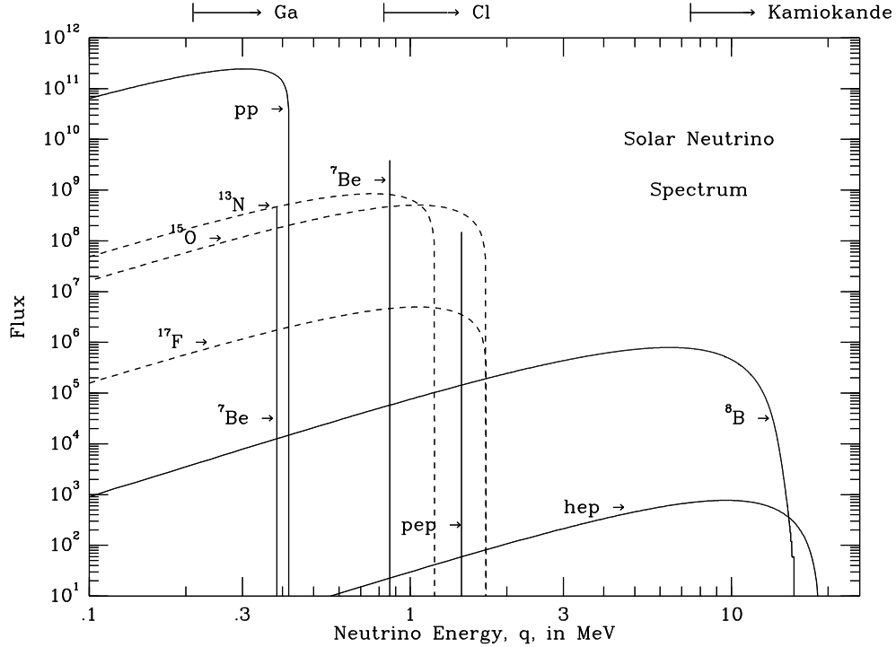
FIG. 1. Solar Neutrino Spectrum. This figure shows the energy spectrum of neutrinos predicted by the standard solar model 3 . The neutrino fluxes from continuum sources (like pp and {}^8\text{B} ) are given in the units of number per \text{cm}^2 per second per MeV at one astronomical unit. The line fluxes (pep and {}^7\text{Be} ) are given in number per \text{cm}^2 per second. The spectra from the pp chain are drawn with solid lines; the CNO spectra are drawn with dotted lines. The arrows at the top of the figure indicate the energy thresholds for the ongoing neutrino experiments.
